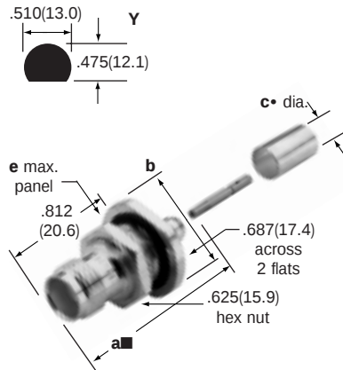
TNC Crimp Type Bulkhead Jack 31-2318 31-2264 31-2389 31-2264-RFX 31-2389-RFX
