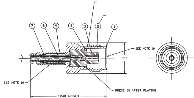
Cable Jack Assembly 79600 31-2317
