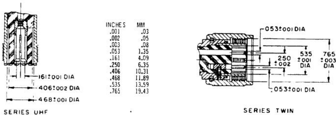
FIGURE 1 Type UG-970/U connector adapter
