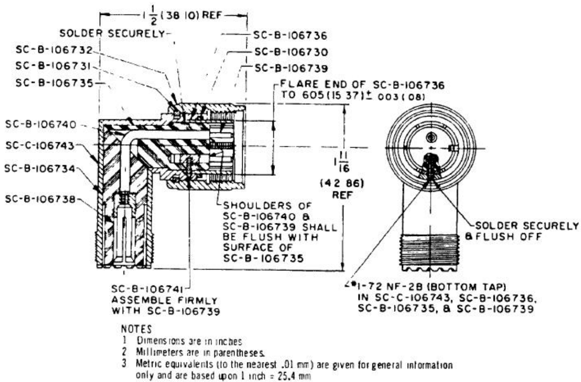
FIGURE 1 Type UG-970/U connector adapter
