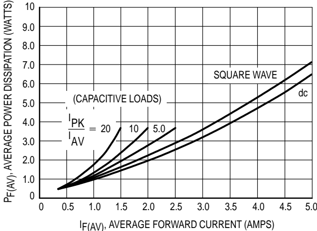
Figure 8. Power Dissipation
