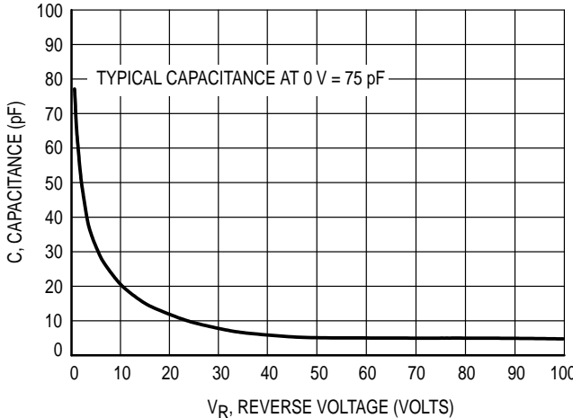
Figure 10. Typical Capacitance
