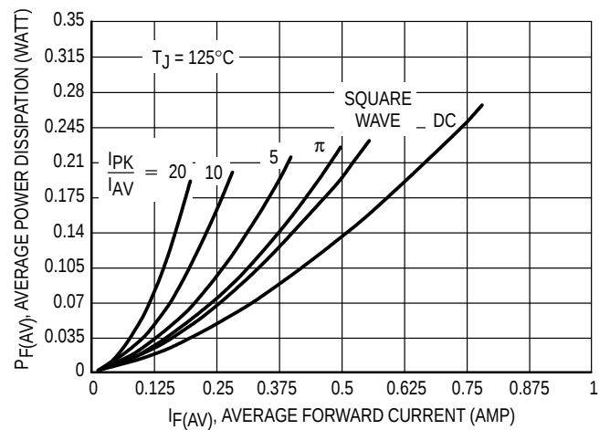
Figure 6. Power Dissipation
