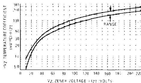
FIGURE 3 – TEMPERATURE COEFFICIENT-RANGE FOR UNITS 10 TO 220 VOLTS
