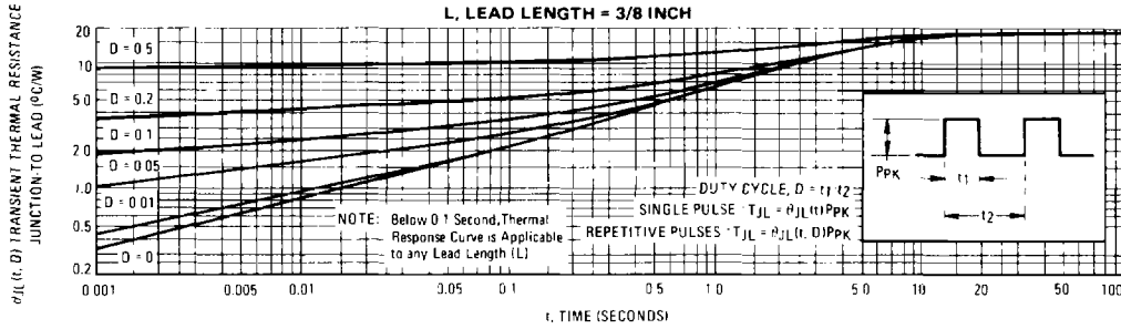
FIGURE 5 – TYPICAL THERMAL RESISTANCE
