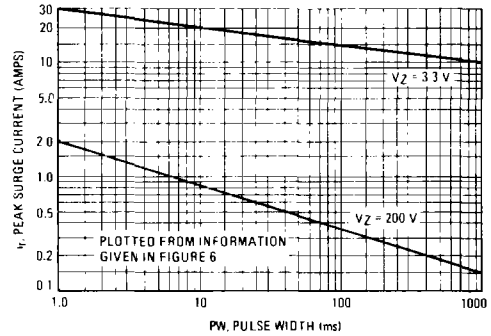
FIGURE 7 – PEAK CURRENT versus PULSE WIDTH (See Note 4)
