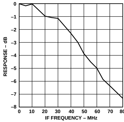
Figure 4. Mixer IF Port Bandwidth
