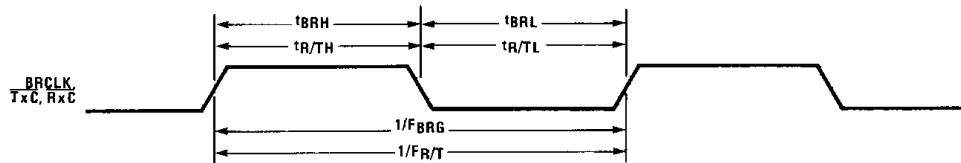
CLOCK TIMING
