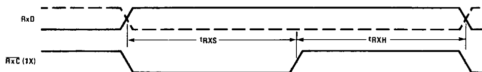
RECEIVE TIMING
