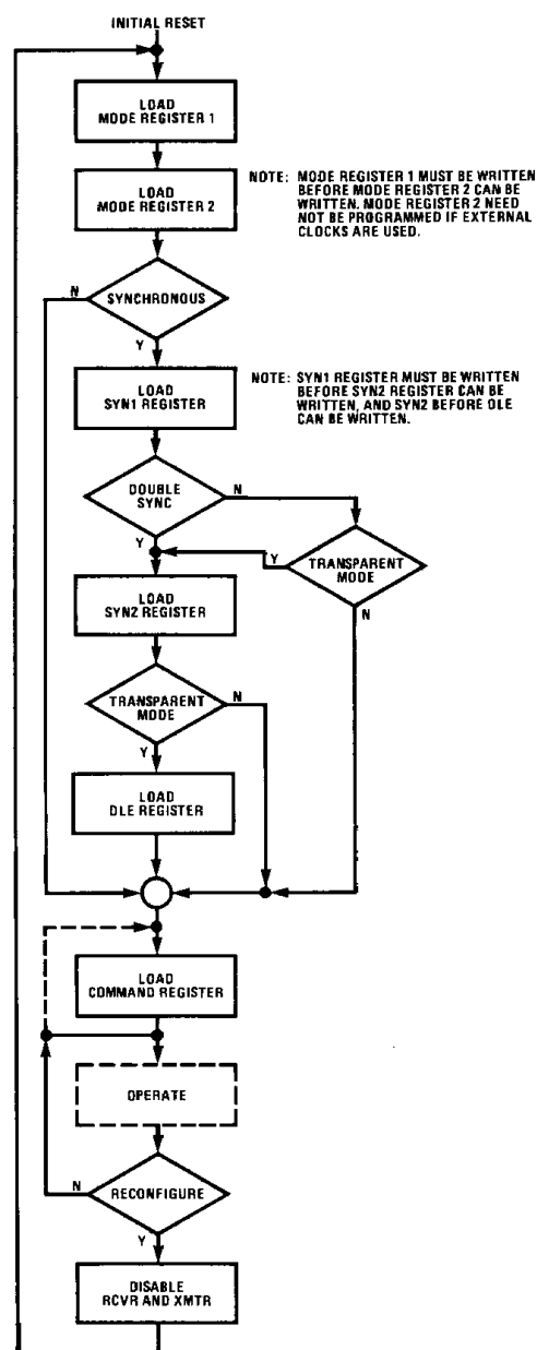
Figure 1. Initialization Flowchart
