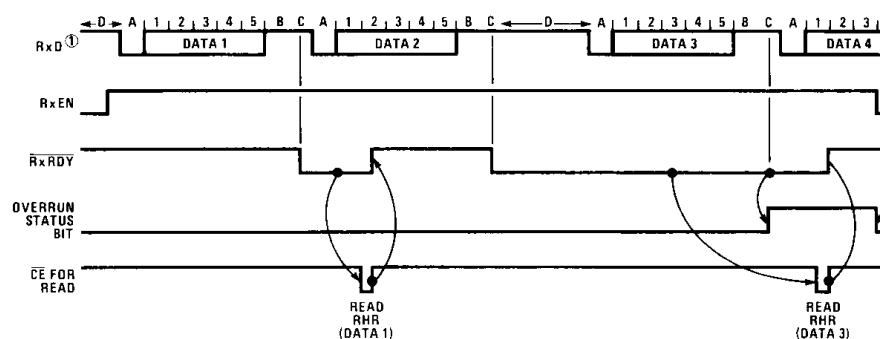
ASYNCHRONOUS MODE
