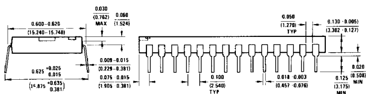
28-Lead Plastic Dual-In-Line Package (N) Order Number INS2651N
