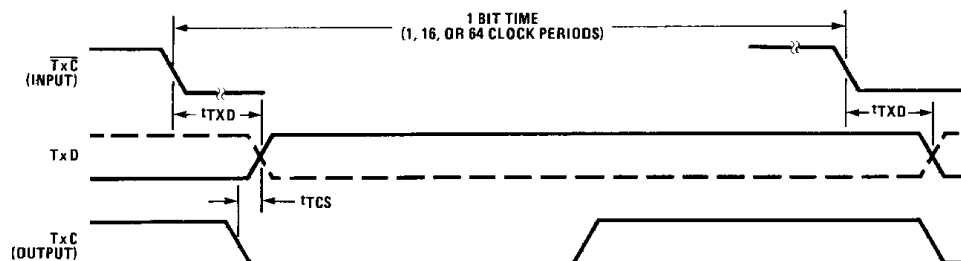
TRANSMIT TIMING
