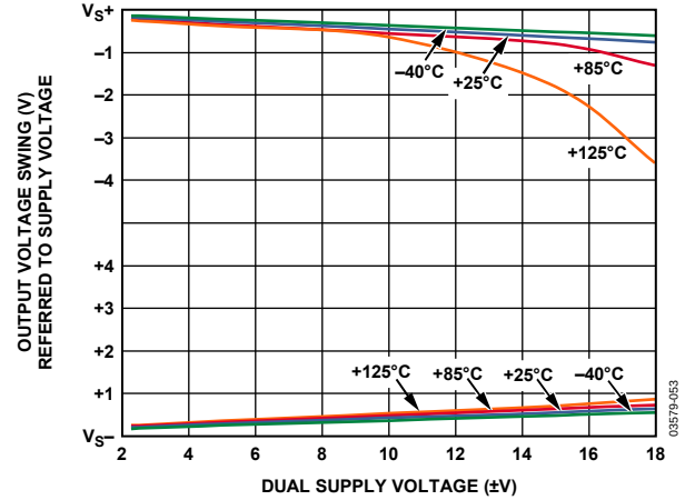
Figure 32. Output Voltage Swing vs. Supply Voltage, R_{LOAD} = 2\text{ k}\Omega , G = 10 , V_{REF} = 0\text{ V}
