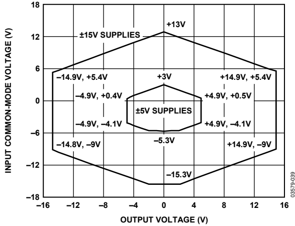
Figure 29. Input Common-Mode Voltage Range vs. Output Voltage, G = 100 , V_{REF} = 0\text{ V}
