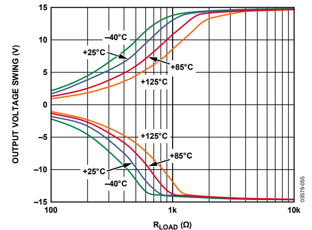
Figure 34. Output Voltage Swing vs. Load Resistance V_S = \pm 15\text{ V} , V_{REF} = 0\text{ V}
