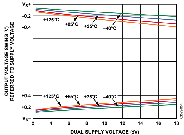
Figure 33. Output Voltage Swing vs. Supply Voltage, R_{LOAD} = 10\text{ k}\Omega , G = 10 , V_{REF} = 0\text{ V}
