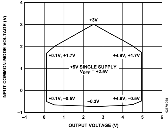
Figure 30. Input Common-Mode Voltage Range vs. Output Voltage, G = 100 , V_S = +5\text{ V} , V_{REF} = 2.5\text{ V}
