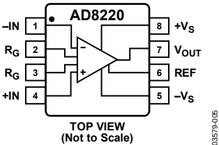
Figure 4. Pin Configuration
