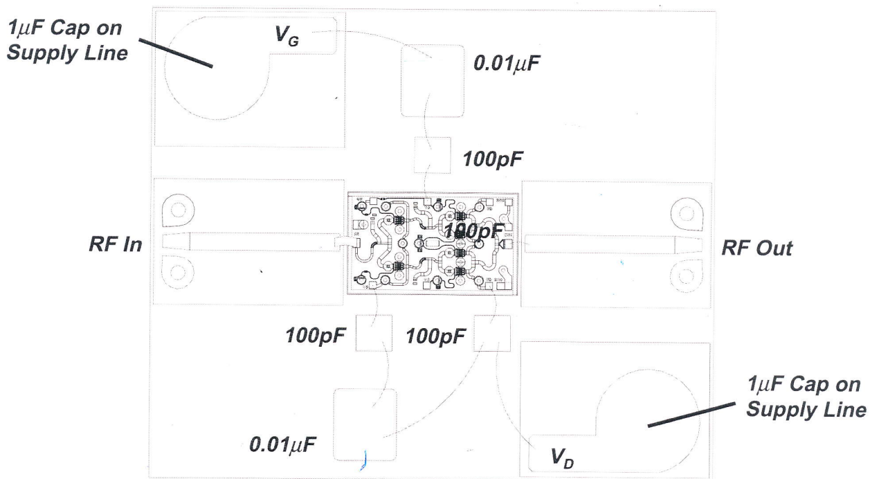
Chip Assembly and Bonding Diagram
