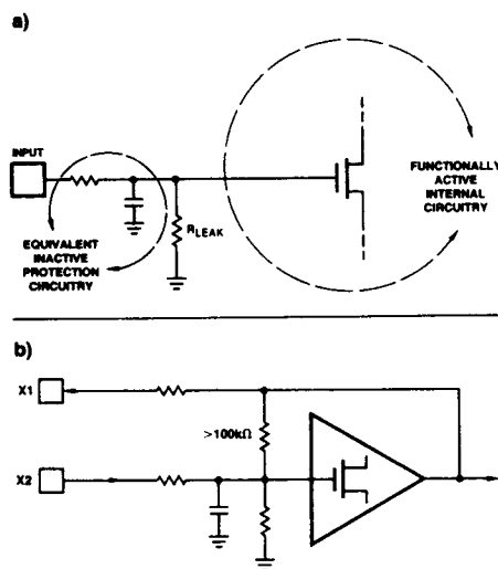
Figure 3. Input Circuitry
