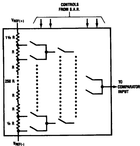
FIGURE 3. Resistor Ladder and Switch Tree
