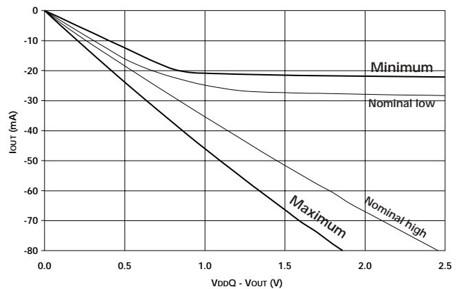
Figure 11: Reduced Drive Pull-Up Characteristics
