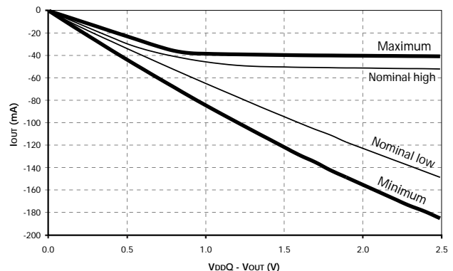
Figure 9: Pull-Up Characteristics
