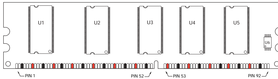
Figure 2: 184-Pin DIMM Pinouts
