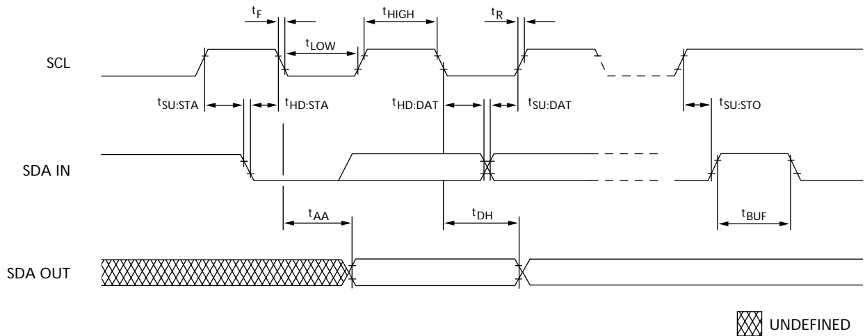
Figure 16: SPD EEPROM Timing Diagram
