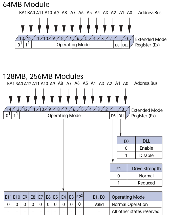
Figure 6: Extended Mode Register Definition Diagram
