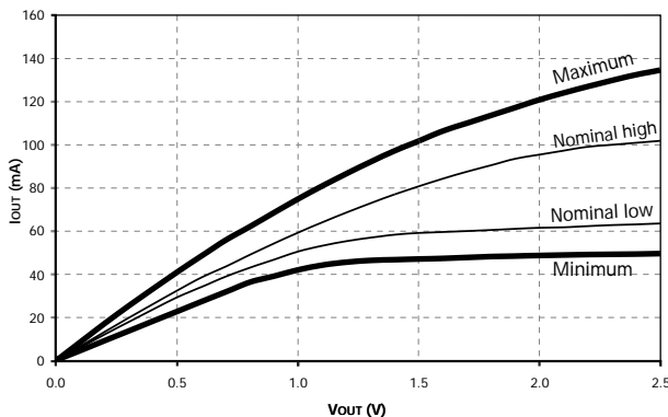
Figure 8: Pull-Down Characteristics
