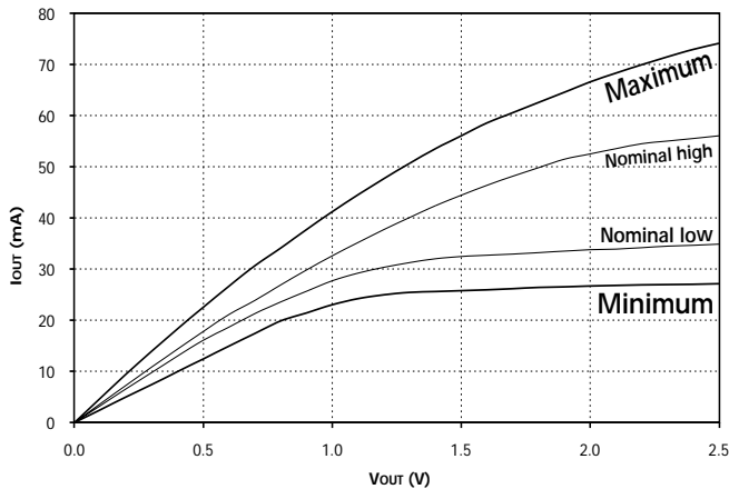
Figure 10: Reduced Drive Pull-Down Characteristics
